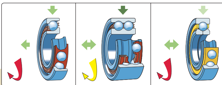
hoekcontactkogellagers
