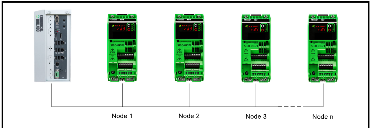
Figure 8-1 System configuration
