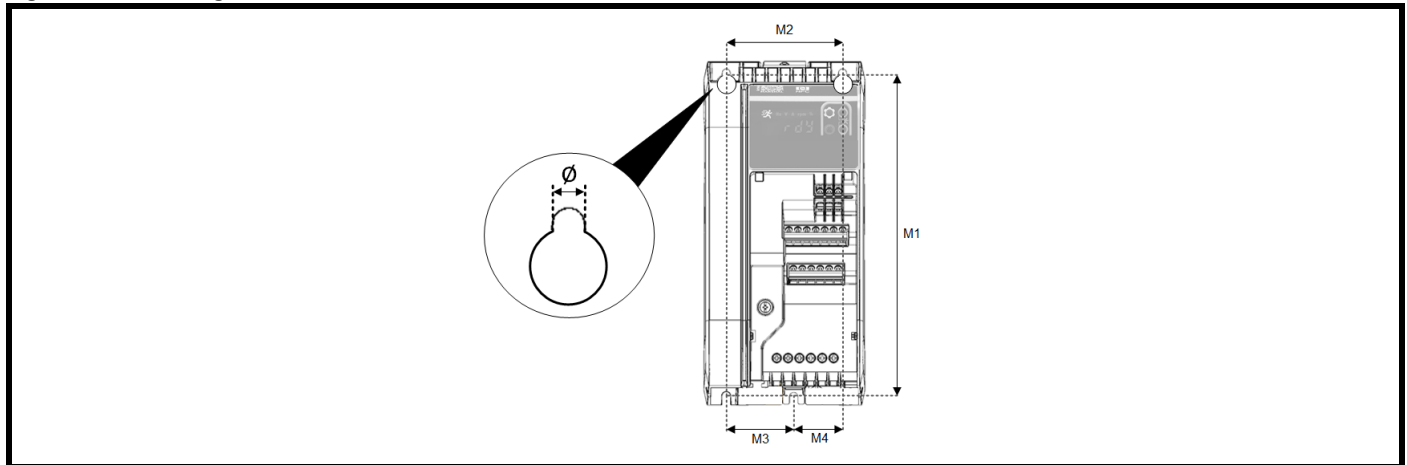
Figure 3-6 Mounting dimensions
